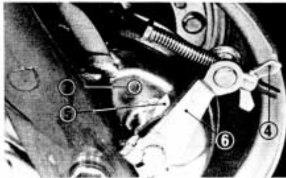
(4) Adjusting nut
