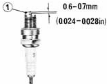
(1) Side electrode
