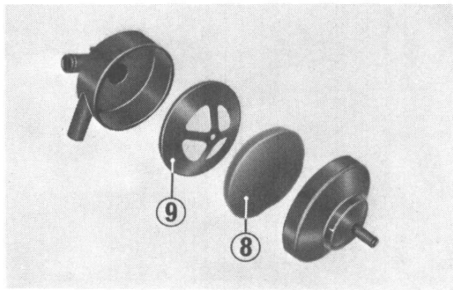
(8) Breather element (9) Element retaining plate
