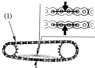
(1) Drive chain
