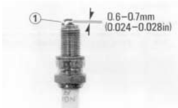
(1) Side electrode
