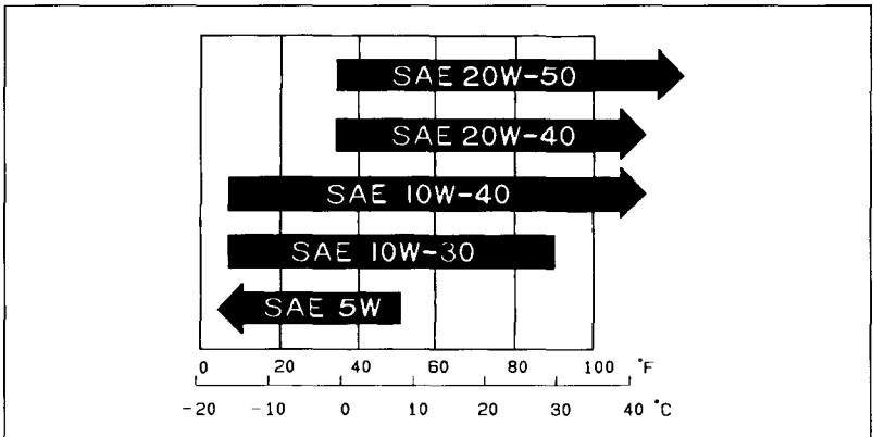
Recommended oil viscosities
