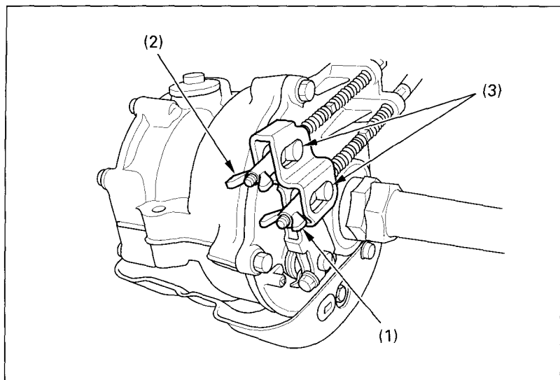
Fig. 4-23 (1) Brake pedal adjusting nut (2) Brake lever adjusting nut
