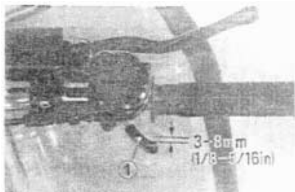
(1) Throttle lever
