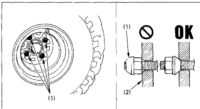
Fig. 4-30 (1) Wheel nuts
