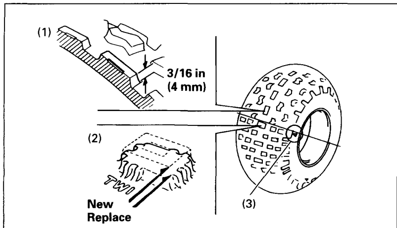
Fig. 4-32 (1) Groove depth (2) Wear indicator
