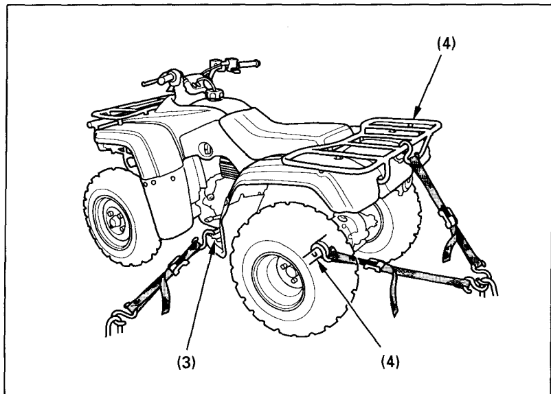
Fig. 4-37 Points to secure FOURTRAX with tie downs
