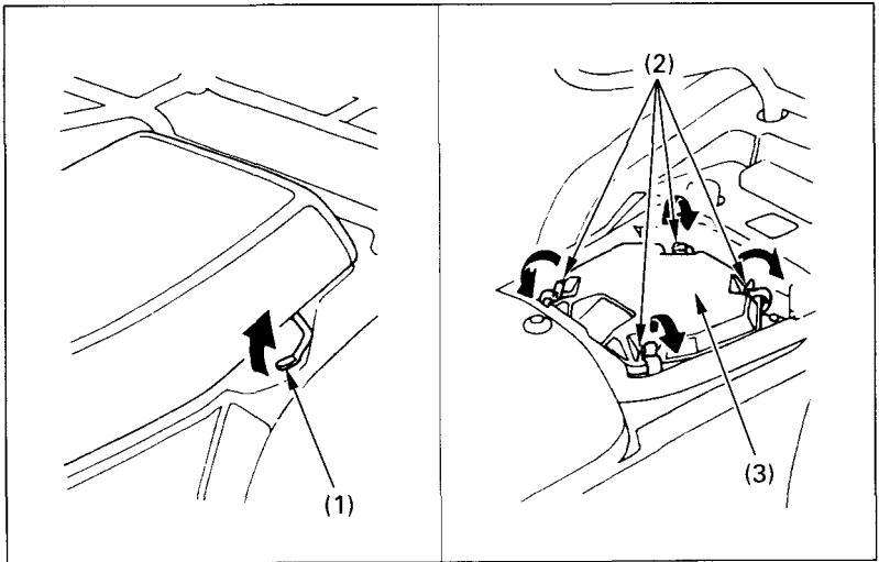
(3) Air cleaner housing cover
