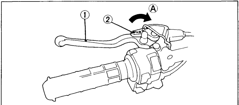
Fig. 2-16 (1) Rear brake lever/Parking brake (2) Lock lever (A) To lock 25
