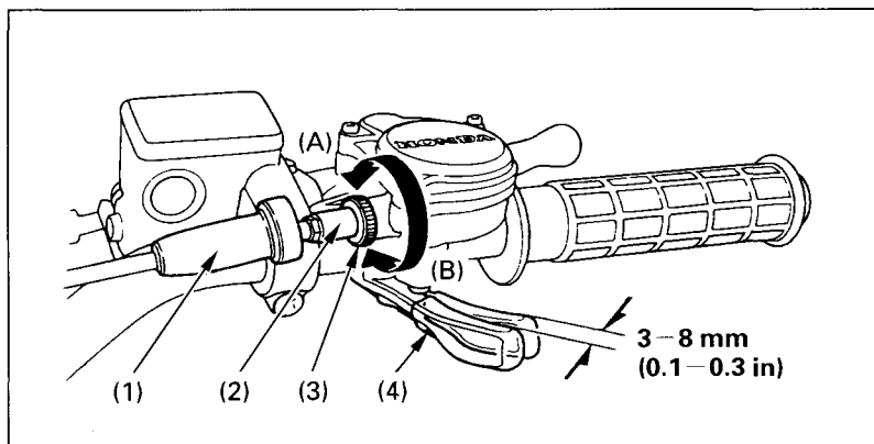
Fig. 4-4 (1) Rubber sleeve (2) Cable adjuster (3) Lock nut (4) Throttle lever (A) To decrease free play (B) To increase free play
