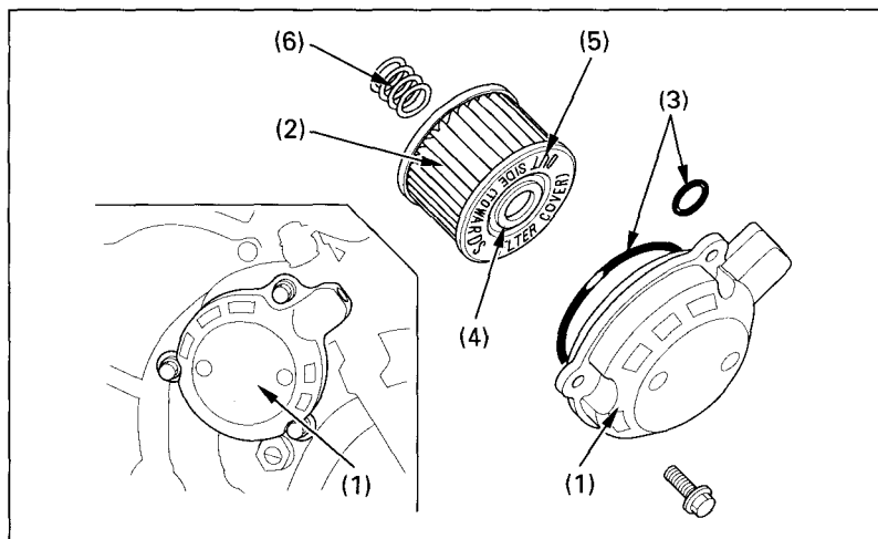
Fig. 4-14 (1) Oil filter cover (2) Oil filter (3) O-rings
