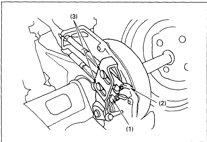
Fig. 4-27 (1) Brake pedal adjusting nut (3) Brake arm pin (2) Brake lever adjusting nut
