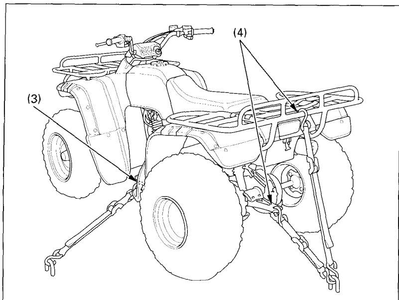
Fig. 4-39 Points to secure FOURTRAX with tie downs
