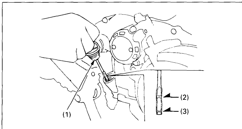
Fig. 4-11 (1) Oil filler cap/dipstick (2) Upper level mark (3) Lower level mark
