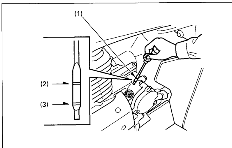
Fig. 2-27 (1) Dipstick
