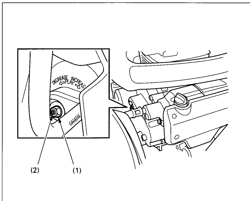
Fig. 4-16 (1) Lock nut
