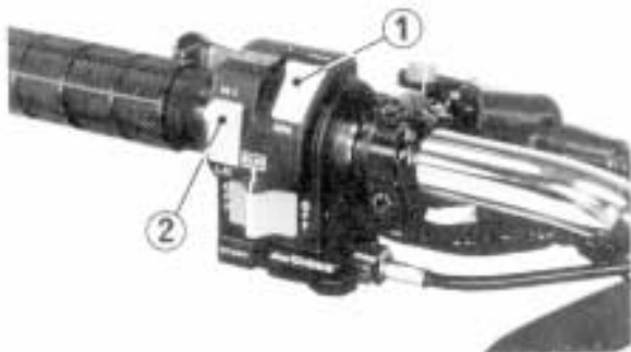
(1) Headlight switch (2) Headlight dimmer switch
