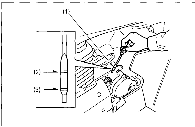
Fig. 2-27 (1) Dipstick
