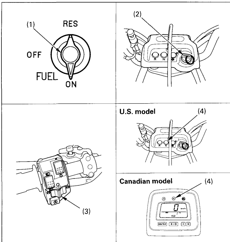
(3) Engine stop switch (4) Neutral indicator
