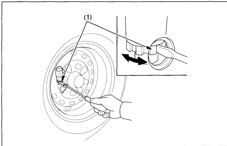
(1) Brake adjusters
