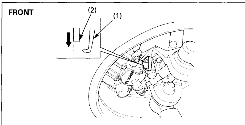
Fig. 4-26 (1) Wear indicator
