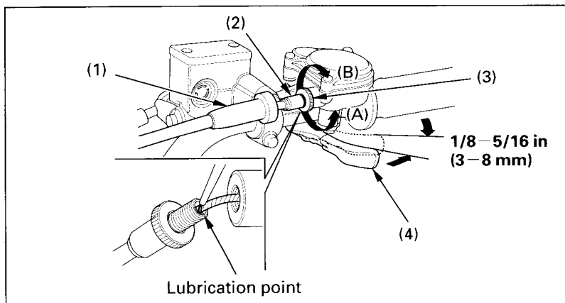
Fig. 4-4 (1) Rubber sleeve (2) Cable adjuster (3) Lock nut (4) Throttle lever (A) To decrease free play (B) To increase free play
