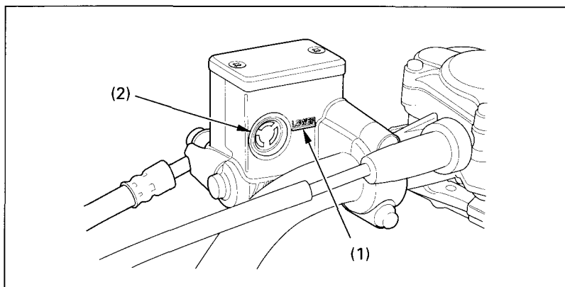
Fig. 4-23 (1) Lower level mark (2) Inspection window
