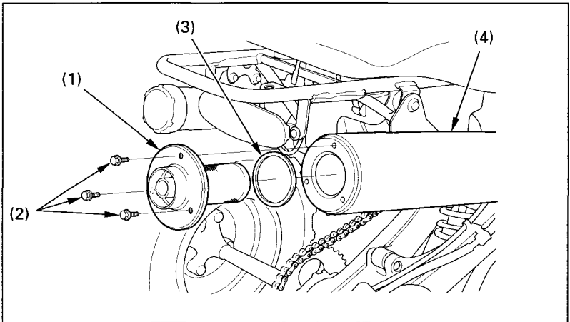
Fig. 4-34 (1) Spark arrester (2) Bolts
