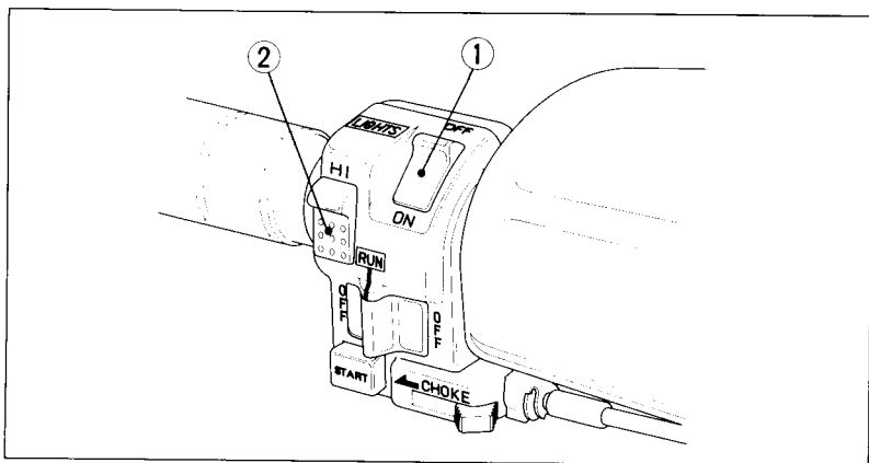
Fig. 2-11 (1) Headlight switch (2) Dimmer switch
