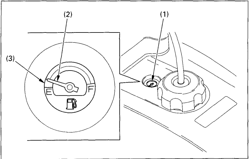
Fig. 2-18 (1) Fuel gauge
