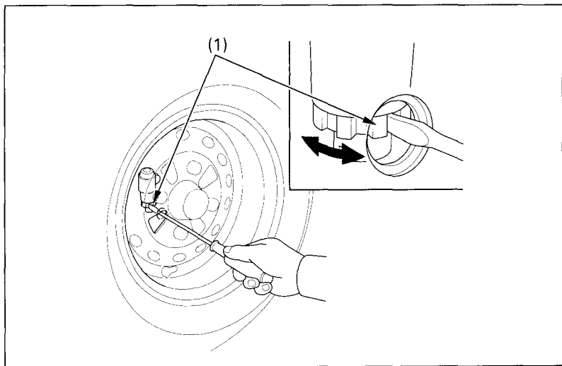
(1) Brake adjusters
