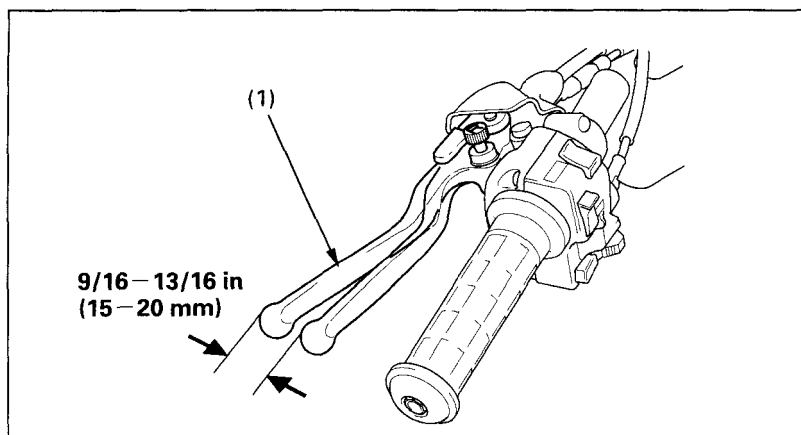
(1) Brake lever
