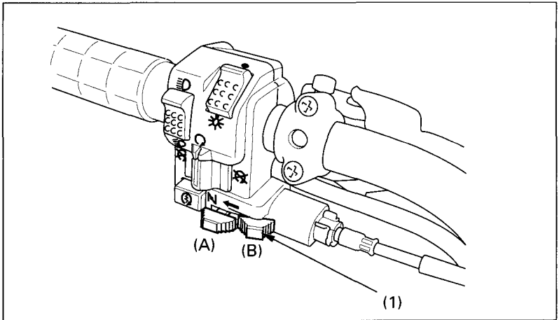
Fig. 2-7 (1) Choke lever
