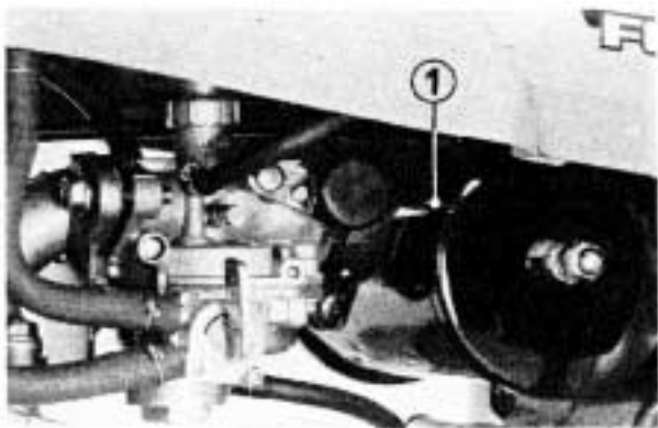
(1) Choke lever
