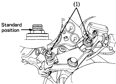
(1) Adjuster
