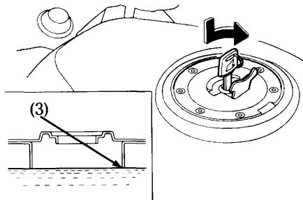
(3) Filler neck
