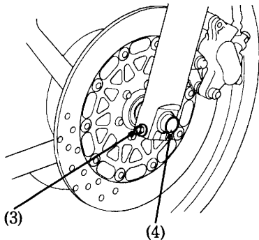
(3) Axle pinch bolts (4) Front axle
