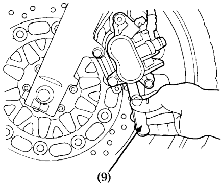
(9) Feeler gauge
