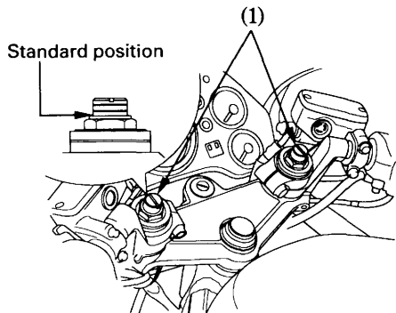
(1) Adjuster
