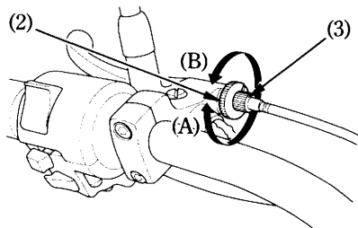
(2) Lock nut
