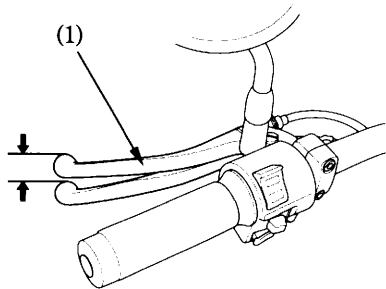
(1) Clutch lever
