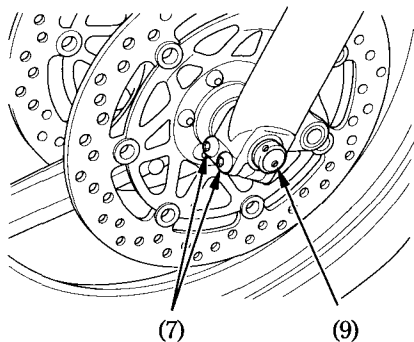
(9) Front axle
