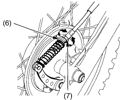
(6) lower lock nut (7) lower adjusting nut
