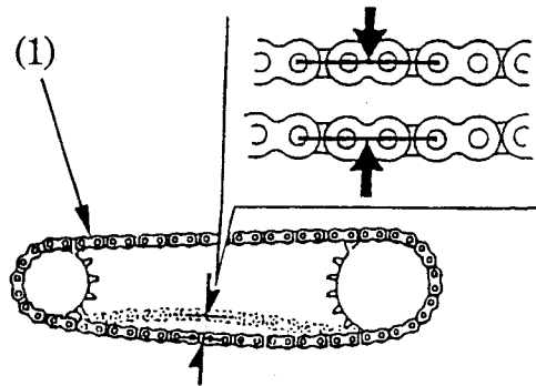
(1) Drive chain
