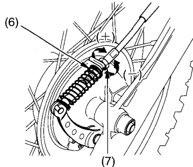
(6) lower lock nut (7) lower adjusting nut
