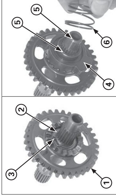
(1) PINION GEAR (2) THRUST WASHER (3) SNAP RING (4) STARTER RATCHET (5) PUNCH MARKS (6) RATCHET SPRING
