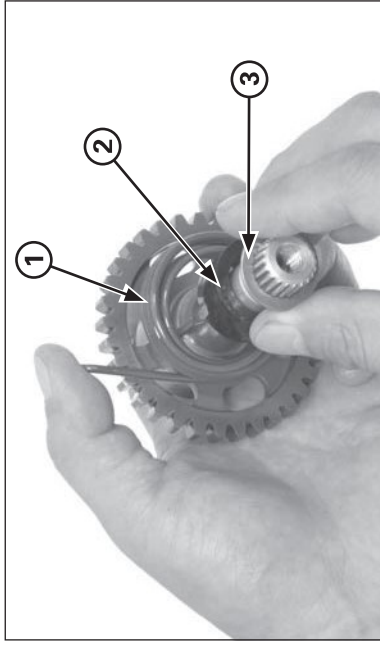
(1) RETURN SPRING (2) COLLAR (3) WASHER
