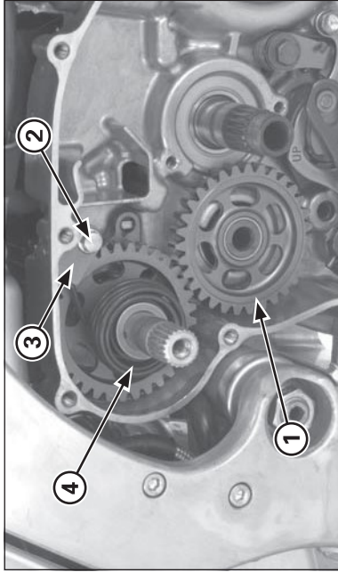
(1) IDLE GEAR/THRUST WASHER (2) BOLT (3) STOPPER PLATE (4) KICKSTARTER ASSEMBLY
