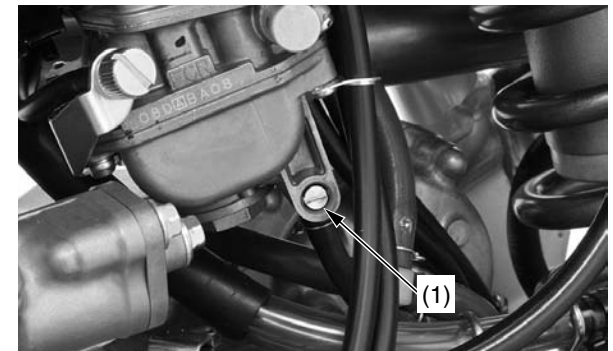
(1) drain screw
