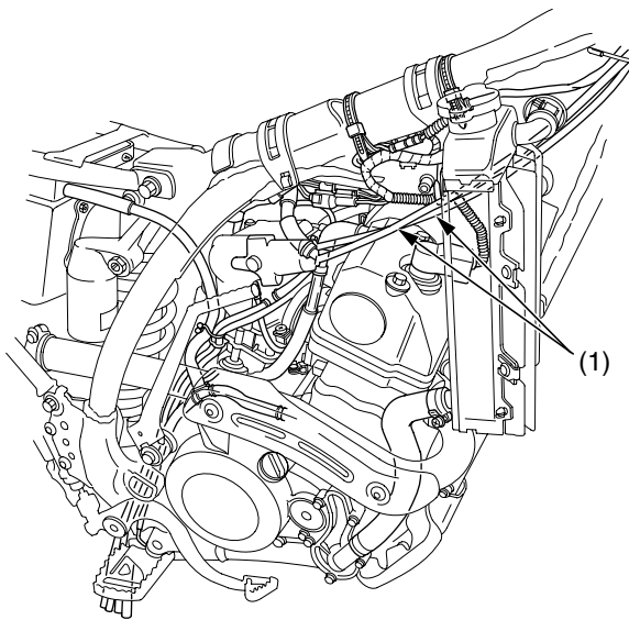
(1) throttle cables
