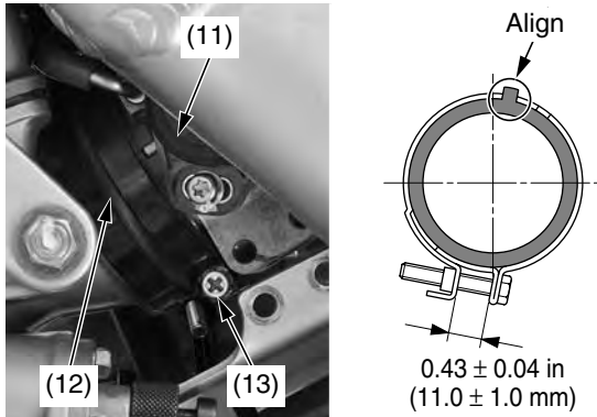
(11) throttle body (12) insulator (13) insulator band screw
