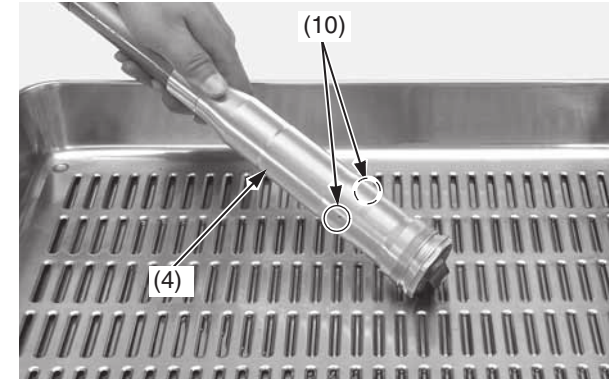
(4) fork damper assembly (10) oil holes
