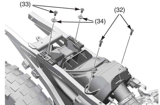
(32) air cleaner housing mounting bolts A (33) air cleaner housing mounting bolts B (34) collars
