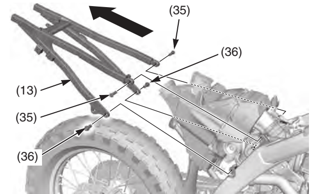
(13) sub frame (35) upper mounting bolts (36) lower mounting bolts
